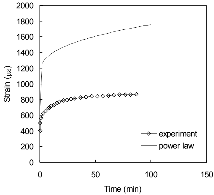
Fig 4.5: Comparison of viscoelastic power law model and representative coupon at 65°C and \sigma_{max}=30\%S_{ut} with R=0.1 . Power law model time is multiplied by a_T(T) according to the time shift factor of Eq. (3.24), for comparison with experimental data.
