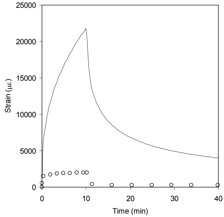
Fig. 3.9: Comparison of representative coupon with DMA time shift factor applied to power law with \sigma_o=43\% Sut at 65^\circ\text{C} .
