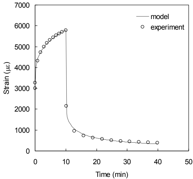
Fig 4.6: Comparison between power law model for HDPE and representative coupon. D_o=.783 \text{ Gpa}^{-1} ( 5.4 \text{ Msi}^{-1} ) D_I=.333 \text{ Gpa}^{-1}\text{min}^{-n} ( 2.3 \text{ Msi}^{-1}\text{min}^{-n} ) n=0.30 , \sigma_o=3.17\text{MPa} .
