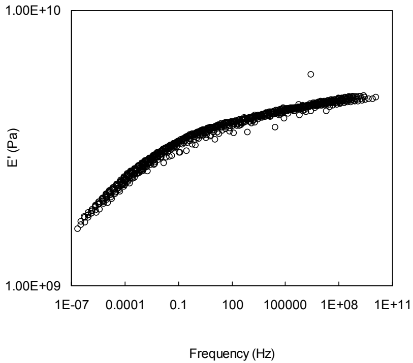
Fig. 3.6: Master curve created using experimentally developed shift factors from DMA.
