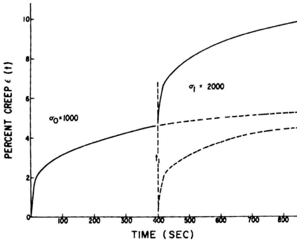
Fig 1.2: Diagram of the Boltzman Superposition Principle [9].
