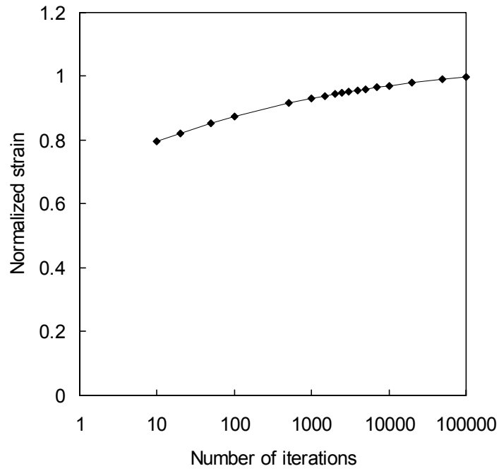
Fig 3.19: Convergence of Simpson's rule for evaluation of Prony Series model incorporating damage.
