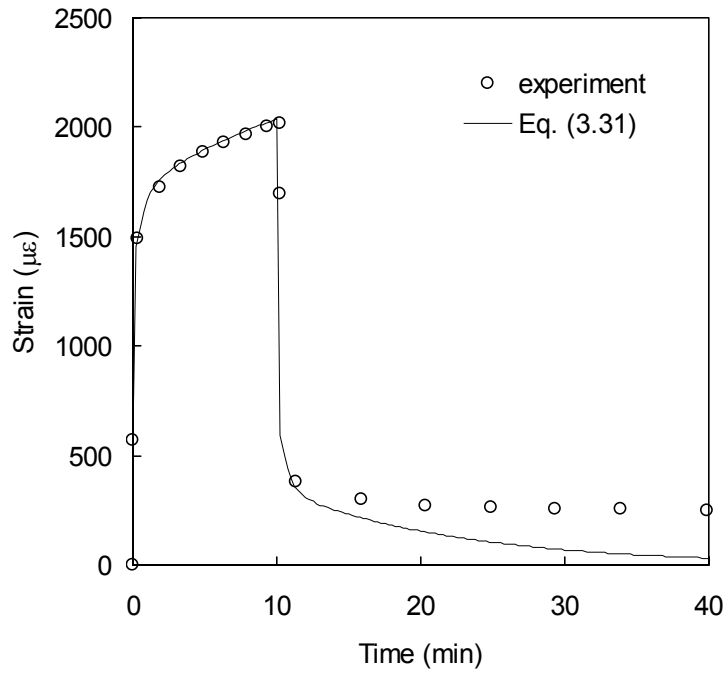
Fig 3.15: Comparison of Prony Series model with representative coupon with \sigma_o=43\% Sut at 65^\circ\text{C} .
