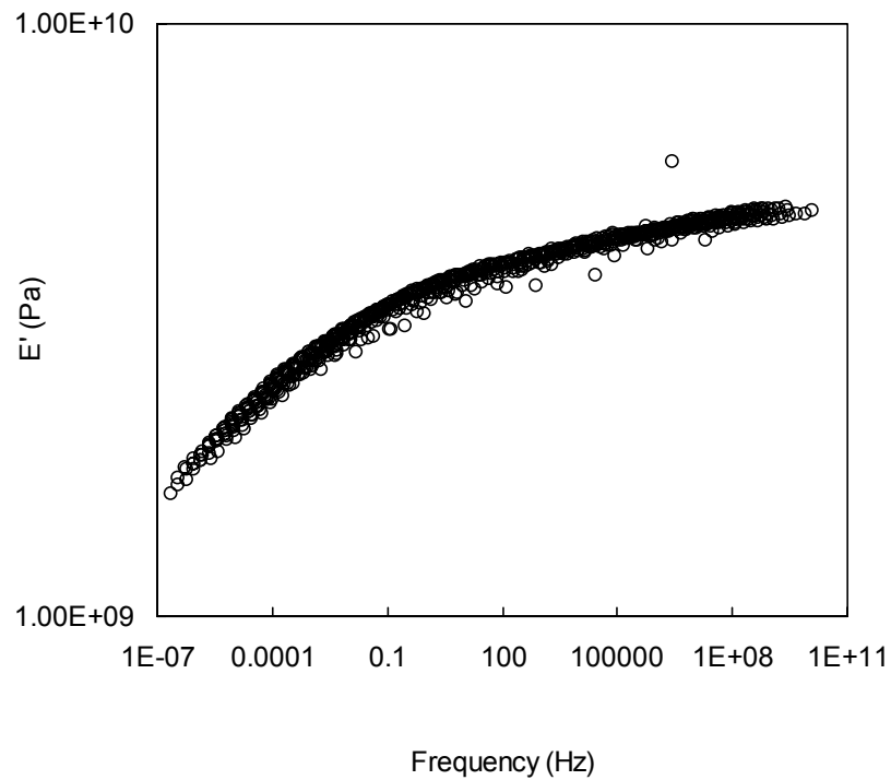
Fig. 2.11: DMA master curve created with WLF shift factors for representative specimen.
