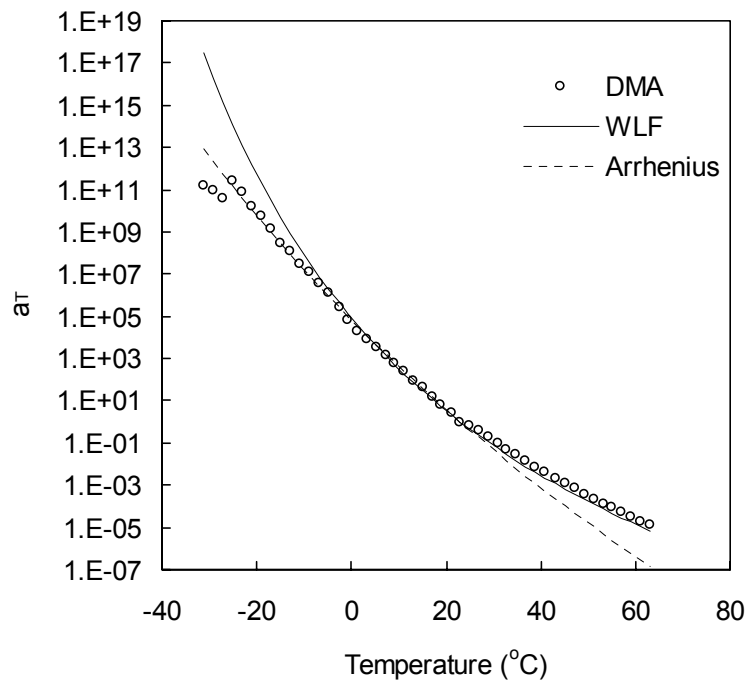
Fig. 2.10: Comparison of experimental DMA, Arrhenius, and WLF time shift factors.
