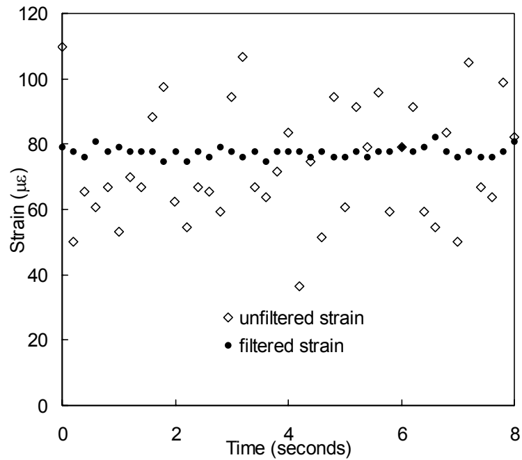
Fig. 2.2: Filtered strain response vs. unfiltered strain response.
