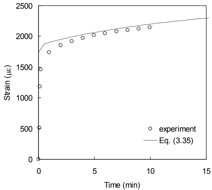
Fig 3.20: Comparison of Prony Series model with representative coupon in creep at \sigma_0=50\% Sut at 23^\circ\text{C} .
