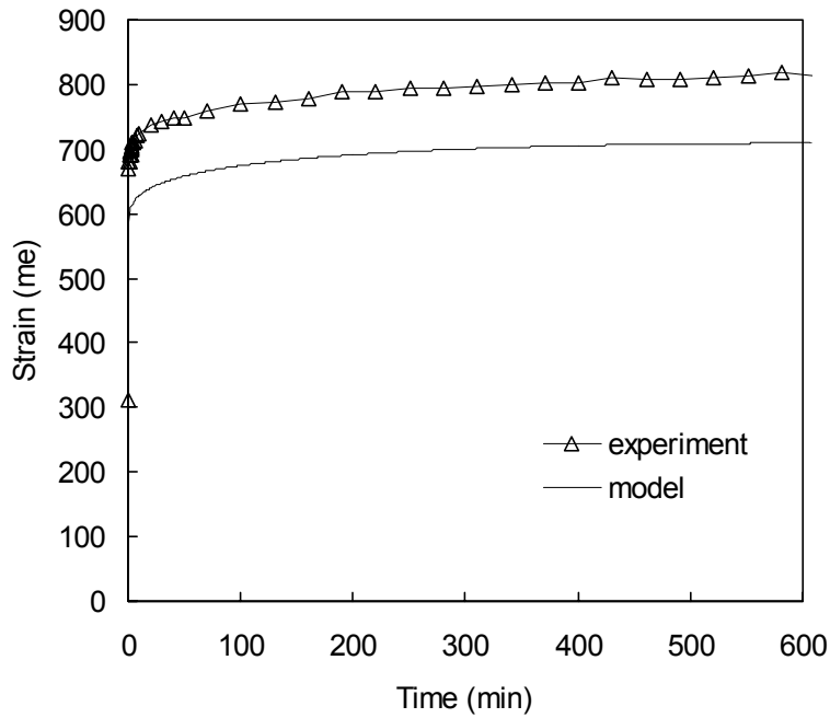
Fig 4.9: Comparison of PP WPC power law fatigue model and representative coupon, \sigma_{max}=3.17\text{MPa} with R=0.1 , f=0.5 Hz.
