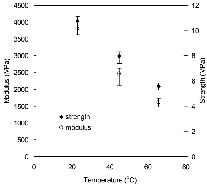
Fig. 2.7: Temperature dependent strength and elastic modulus.
