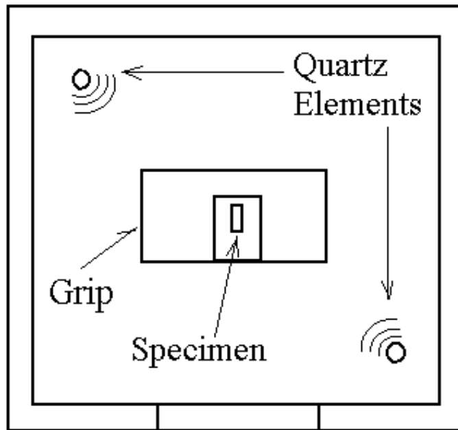
Fig. 2.3: Top view of oven showing placement of heating elements.
