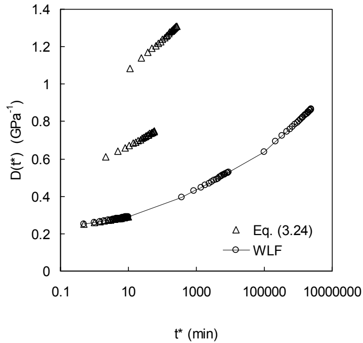
Fig. 3.8: Comparison of representative coupon master curve fit with preliminary horizontal and vertical shift factors used in Eq. (3.24) and a WLF horizontal shift determined by DMA.
