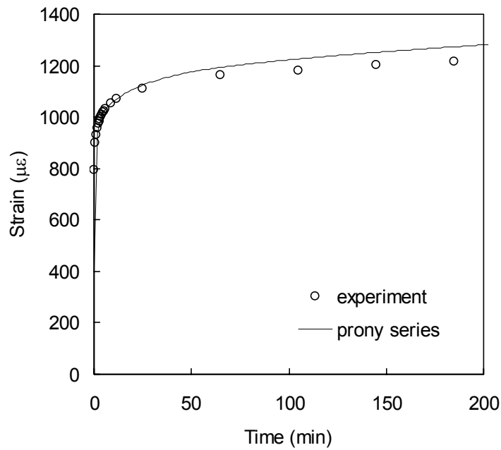
Fig. 4.16: Comparison of representative coupon and Prony Series model at 45°C and \sigma_{max}=30\%S_{ut} with R=0.1 . Shifted time from Fortran model is multiplied by a_T to compare with real time measured experimentally.
