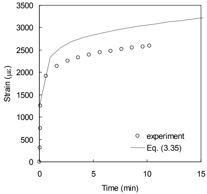
Fig 3.23: Comparison of Prony Series model with representative coupon in creep at \sigma_o=50\% Sut at 45^\circ\text{C} .
