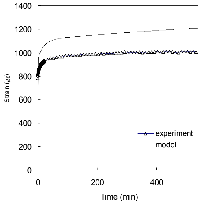
Fig 4.14: Comparison of Prony Series model with experimental data at 23°C and \sigma_{max}=30\%S_{ut} with R=.1 .
