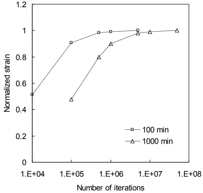
Fig 4.13: Convergence study for Prony Series fatigue model.
