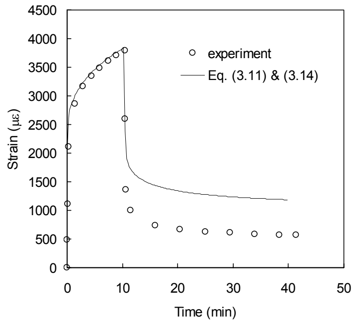
Fig 3.2: Comparison of power law model with damage with experimental data for representative coupon with \sigma_0=70\%Sut at 23^\circ C .
