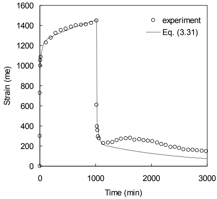
Fig 3.17: Comparison of representative coupon with Prony Series model with \sigma_o=30\% Sut at 23°C. Recovery strain response phenomenon due to lab temperature fluctuation.
