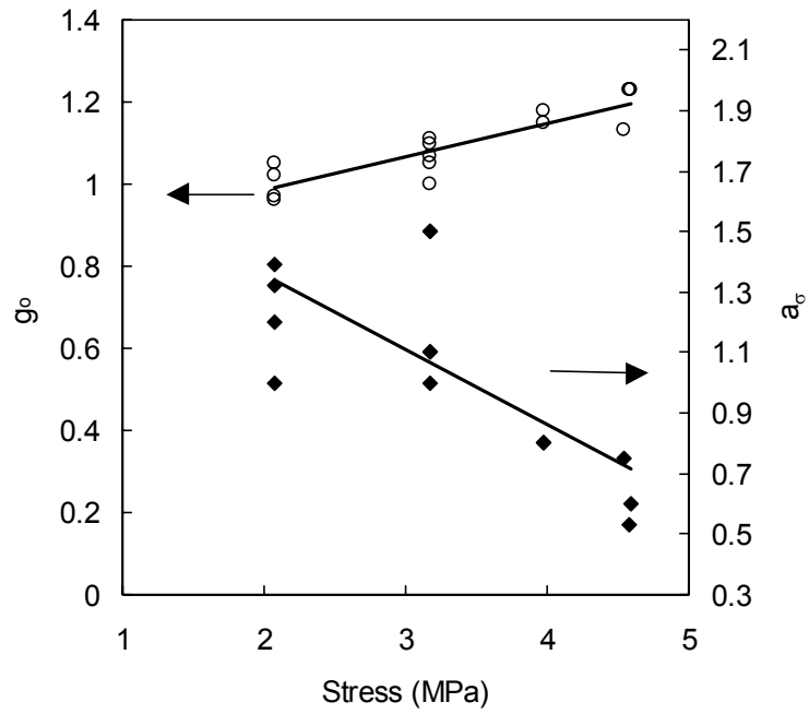
Fig 3.13: Stress dependent parameters for non-linear Prony Series model.
