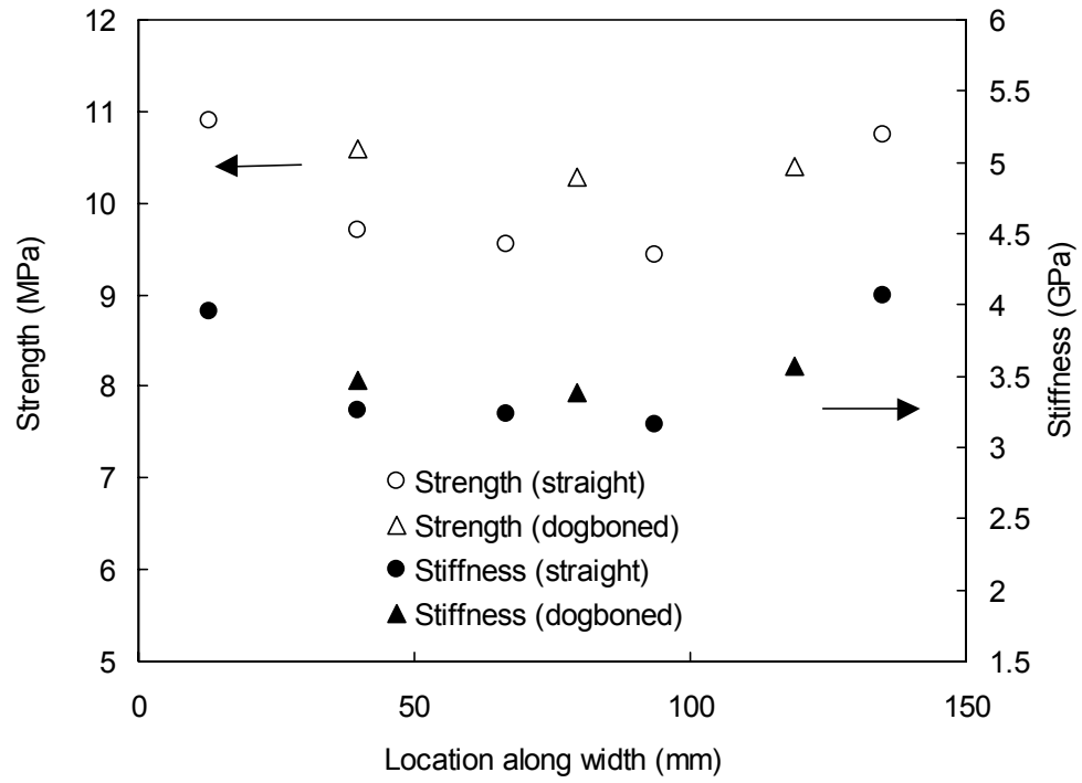
Fig. 2.6: Location dependence of strength and modulus across width of board.
