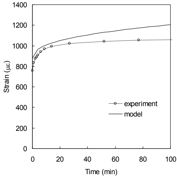
Fig 4.3: Comparison of peak cyclic strains of fatigue model using coupon dependent parameters with experimental data, R=0.1 , \sigma_{max}=30\% Sut at 23^{\circ}\text{C} .
