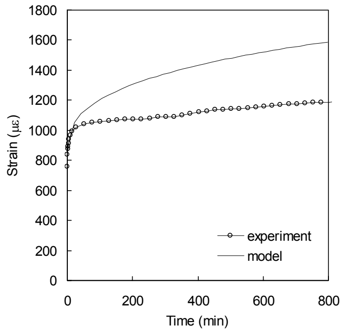
Fig 4.4: Same coupon as Fig. 4.3 showing 800 minutes of data for comparison.
