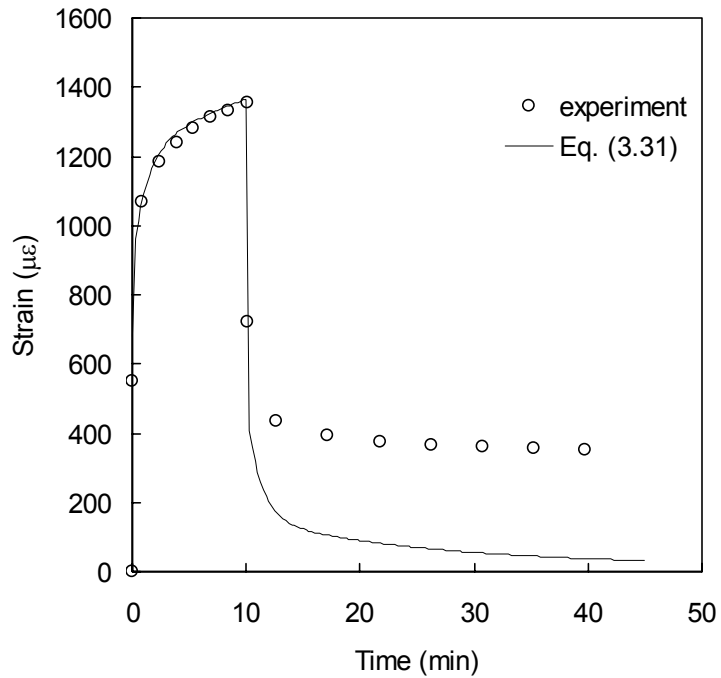
Fig 3.16: Comparison of representative coupon with Prony Series model at \sigma_o=30\% Sut at 45^\circ\text{C} . Extensometer slippage is seen in recovery.
