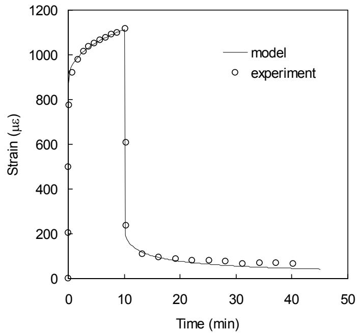
Fig 4.2 Comparison of power law model to 10 minute creep/recovery data at 30%St, 23°C.
