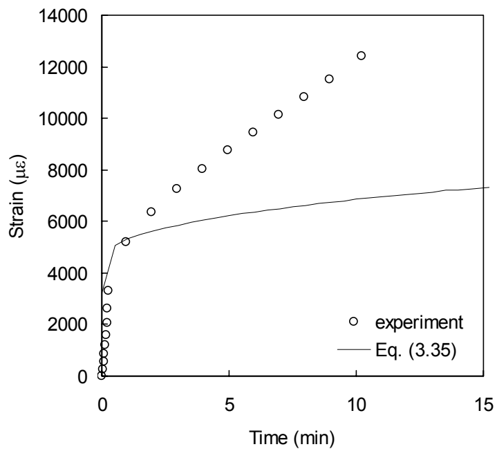
Fig 3.22: Comparison of Prony Series model with representative coupon at \sigma_0=90\% Sut at 23^\circ\text{C} .
