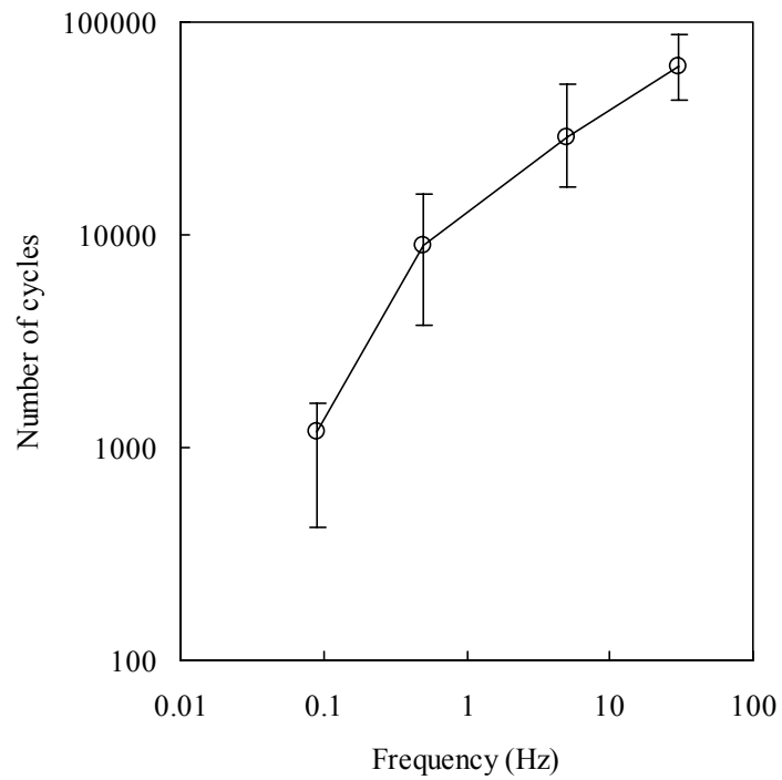
Fig. 2.9: Dependence of fatigue life on fatigue frequency; R=.1 , \sigma_{max}=80\%S_{ut} at 23°C.
