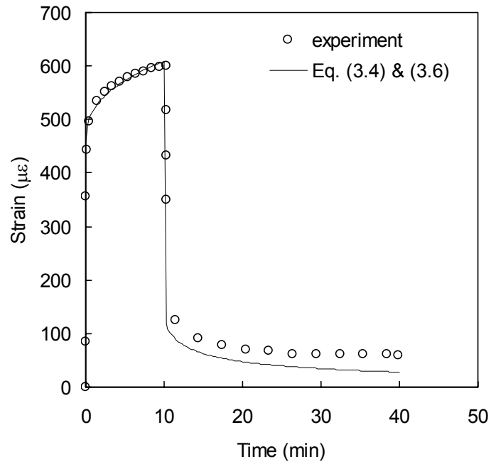
Fig. 3.1: Comparison of power law model with experimental data, \sigma_0=20\%Sut at 23^\circ C .
