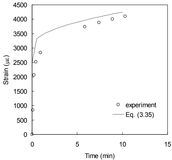
Fig 3.21: Comparison of Prony Series model with representative coupon in creep at \sigma_0=70\% Sut at 23^\circ\text{C} .
