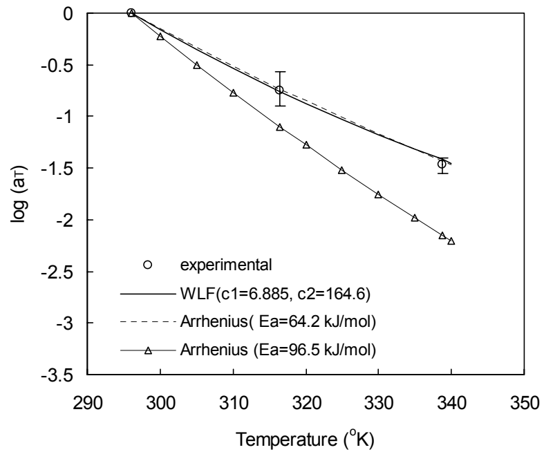
Fig 3.3: Comparison of preliminary shift factors obtained from creep testing with the WLF and Arrhenius relations, where the existence of a vertical shift factor is presumed.
