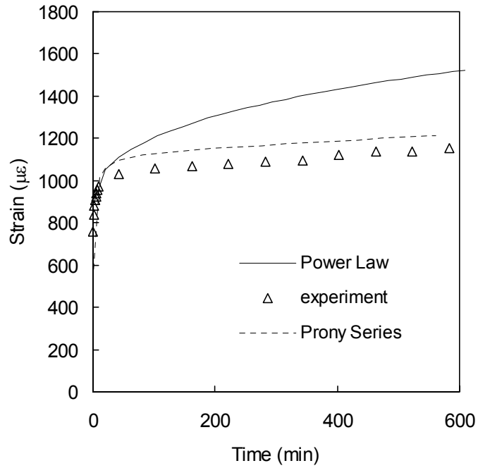
Fig 4.15: Comparison of Prony Series model with power law and experimental data for the coupon shown in Fig 4.3 and 4.4 .
