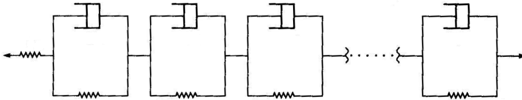
Fig. 1.1: Diagram of a Prony Series [39].
