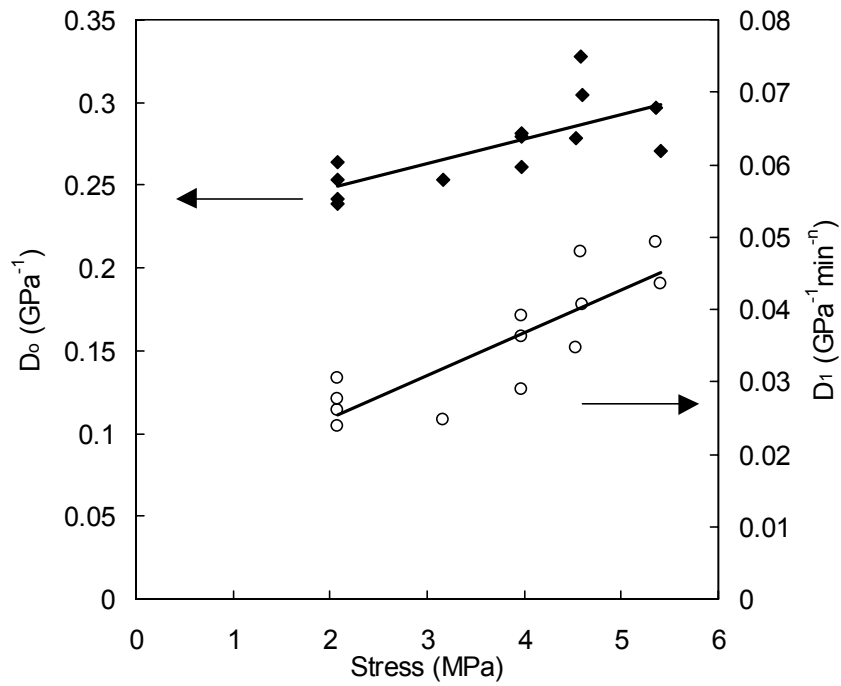
Fig. 3.12: Stress dependence of power law parameters D_0 and D_1 .
