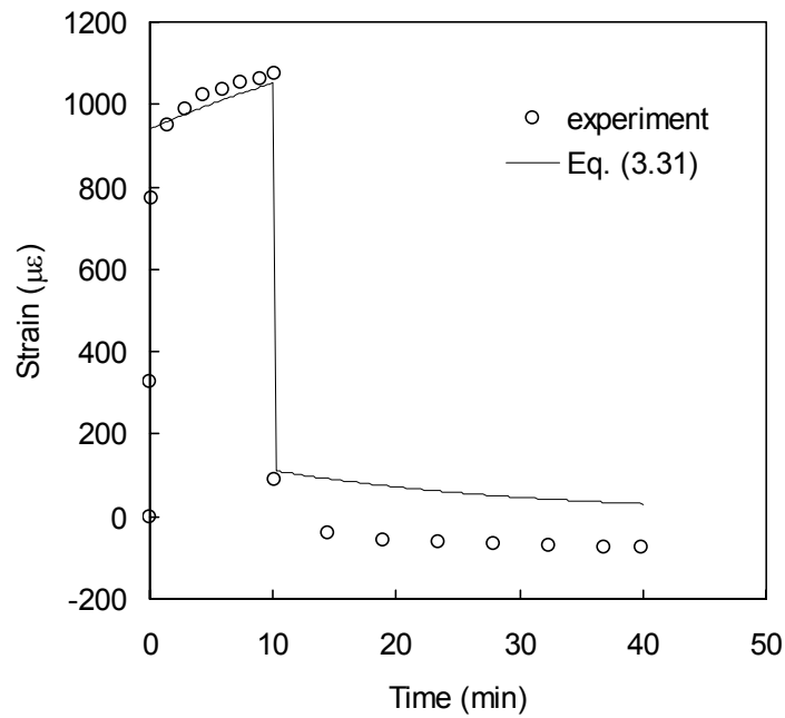
Fig 3.14: Comparison of Prony Series model with representative coupon at 30% Sut at 23°C.
