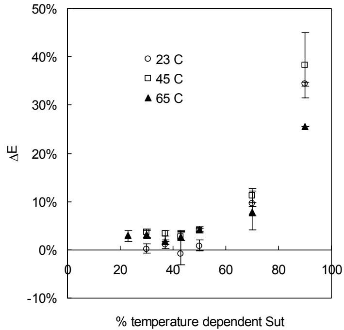
Fig 3.18: Threshold stress determination. \Delta E=1-E_i/E_f where E_f is the final stiffness and E_i is the initial stiffness
