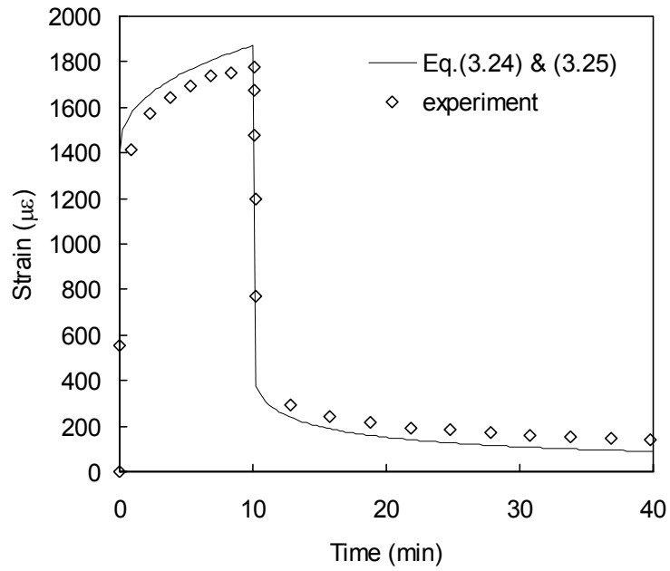
Fig. 3.5: Comparison of Eq. 3.24 and 3.25 with representative coupon with \sigma_o=37\% Sut and T= 65^\circ\text{C} .
