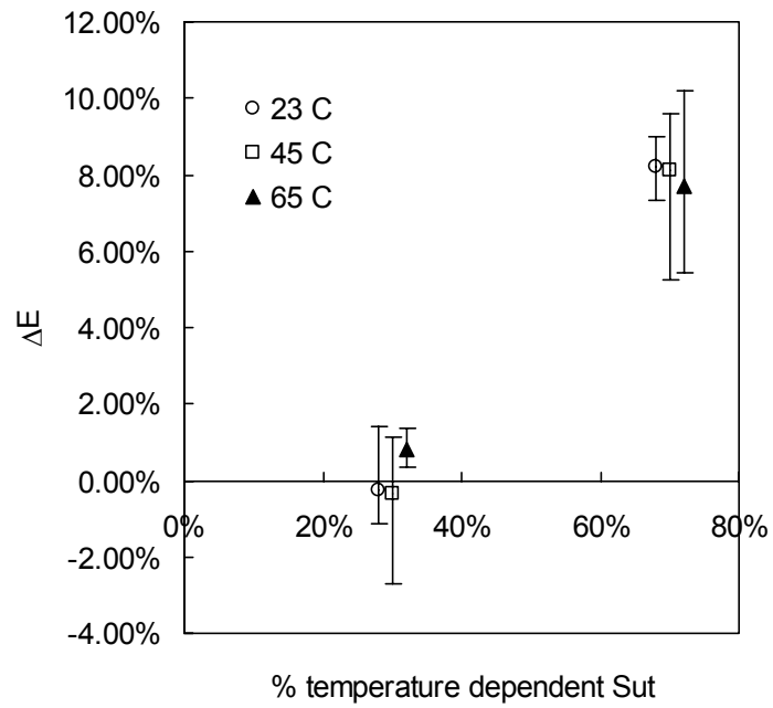
Fig. 4.19: Percent reduction in elastic modulus \Delta E=1-E_i/E_f in fatigue loading where E_f is the final stiffness and E_i is the initial stiffness.
