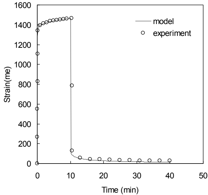
Fig 4.10: Comparison between power law model for PVC WPC and representative coupon. D_o=.13 \text{ Gpa}^{-1} ( 0.9\text{Msi}^{-1} ) D_I=.013 \text{ Gpa}^{-1}\text{min}^{-n} ( .09 \text{ Msi}^{-1}\text{min}^{-n} ) n=0.19 , \sigma_o=9.72\text{MPa} .
