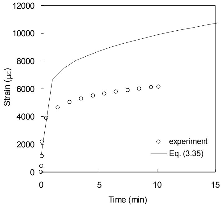
Fig 3.24: Comparison of Prony Series model with representative coupon in creep at \sigma_o=70\% Sut at 65^\circ\text{C} .
