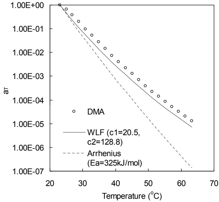
Fig 3.7: Comparison of the shift factor found from DMA with the Arrhenius and WLF equations.
