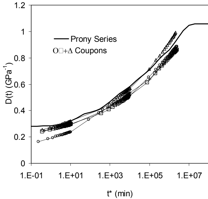
Fig. 3.11: Prony Series comparison with master curves for four coupons at \sigma_0=2.07 MPa. Inherent coupon to coupon variation is evident.
