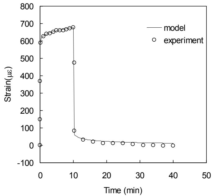
Fig 4.7: Comparison of HDPE power law fatigue model and representative coupon, \sigma_{max}=4.1 MPa with R=0.1, f=0.5 Hz.
