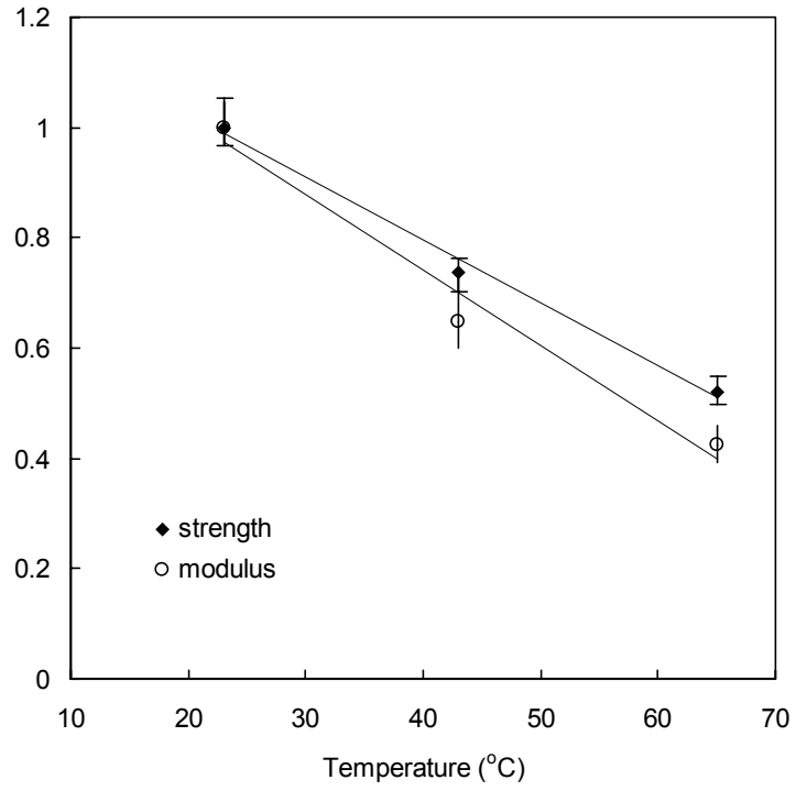
Fig. 2.8: Normalized strength and elastic modulus with strength and elastic modulus at 23°C.
