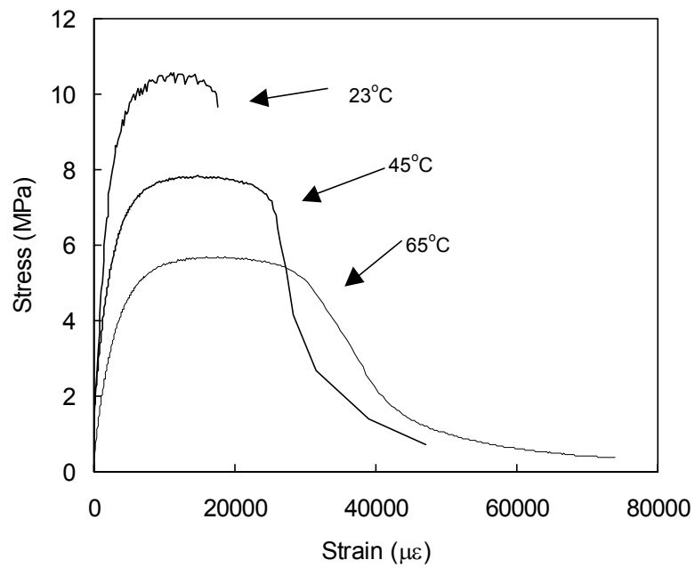
Fig. 2.4: Representative stress-strain curves for coupons at 23°C, 45°C, and 65°C.
