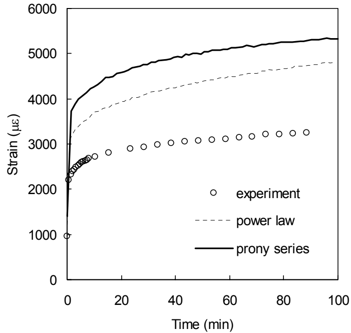
Fig 4.17: Convergence of the power law damage model at 100 minutes. 15,000t iterations required.
