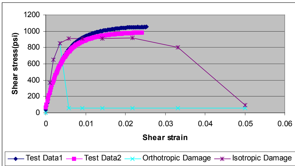
Figure 5-11: Comparison of the pure shear results for the HDPE material model with torsion tests
