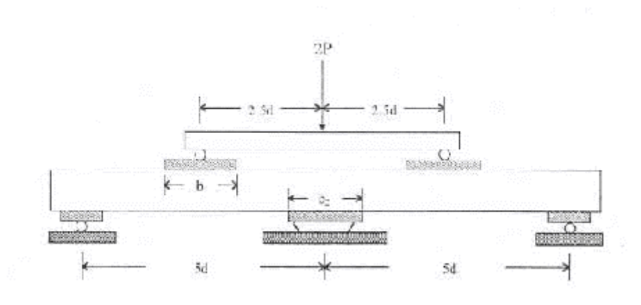
Figure 6-16: Five-point bending shear test setup (Haiar, 2000)
